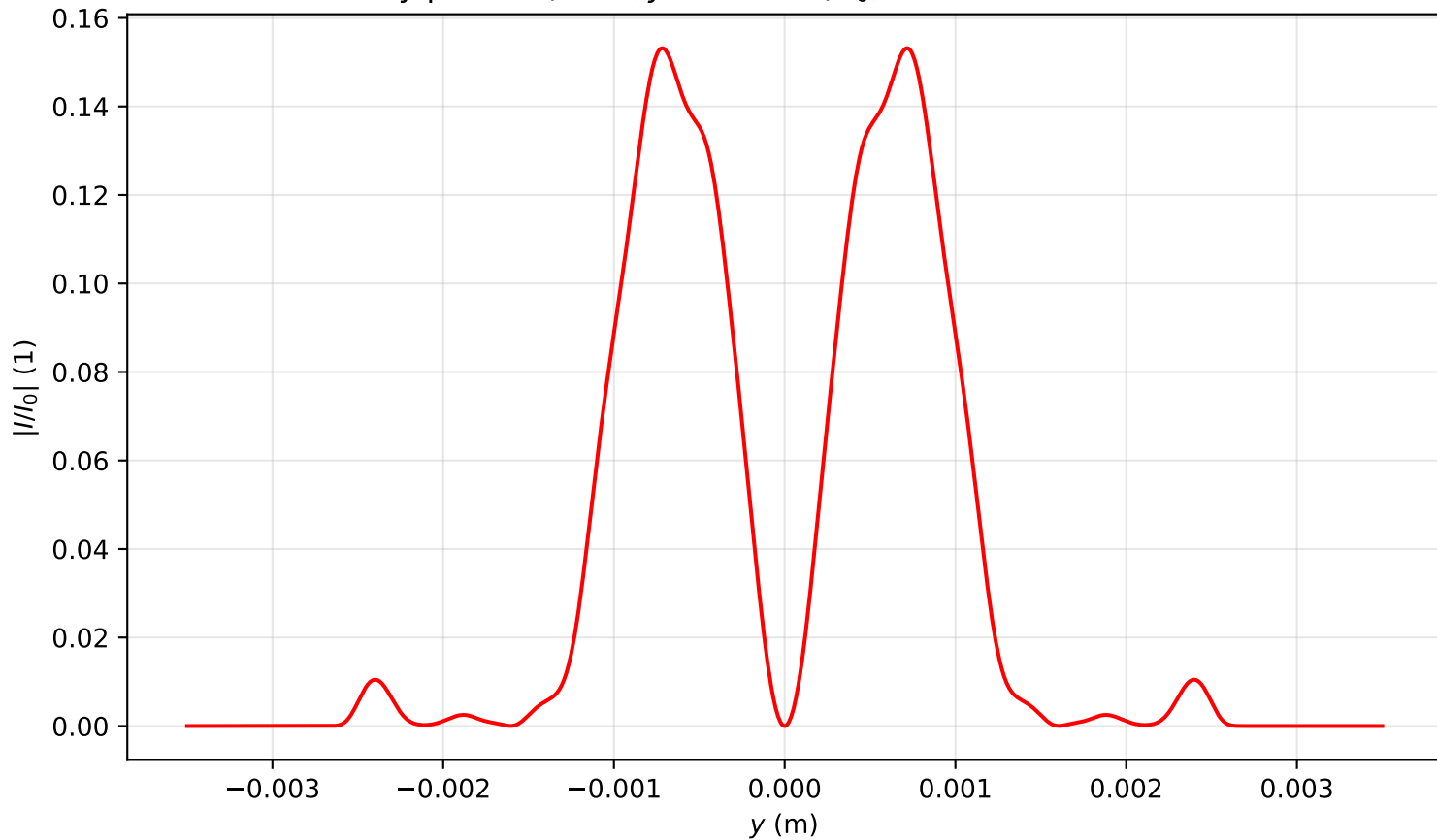
Intensity profile I(x=0, y, z=2.707)/I_0 , P_{in}=7.0P_{cr} , artificial time
